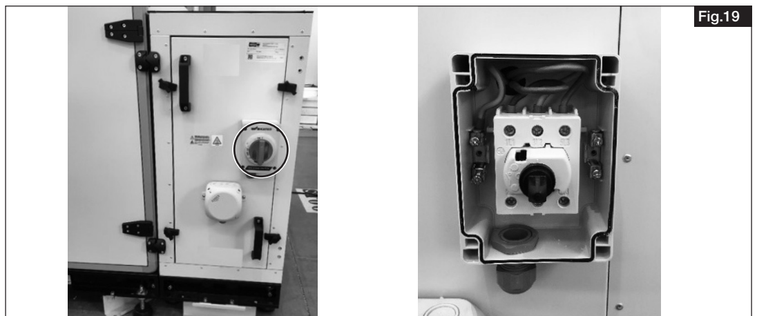
8. Open main switch cover. Check cable thickness for the power connection (see Fig. 19). Connect the cables to the terminals and close the main switch cover.
