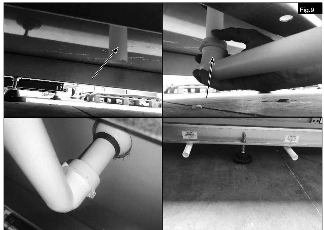
2. Fix the pipe bend below the condensation tray. Ensure that the construction is water-tight by turning the pipe connector (see Fig.9).
