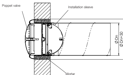
Installation in concrete or aerated concrete, installation sleeve
