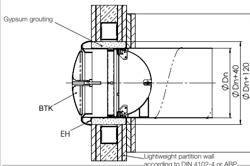
Installation in metal stud walls Insertion in spiral duct, valve
